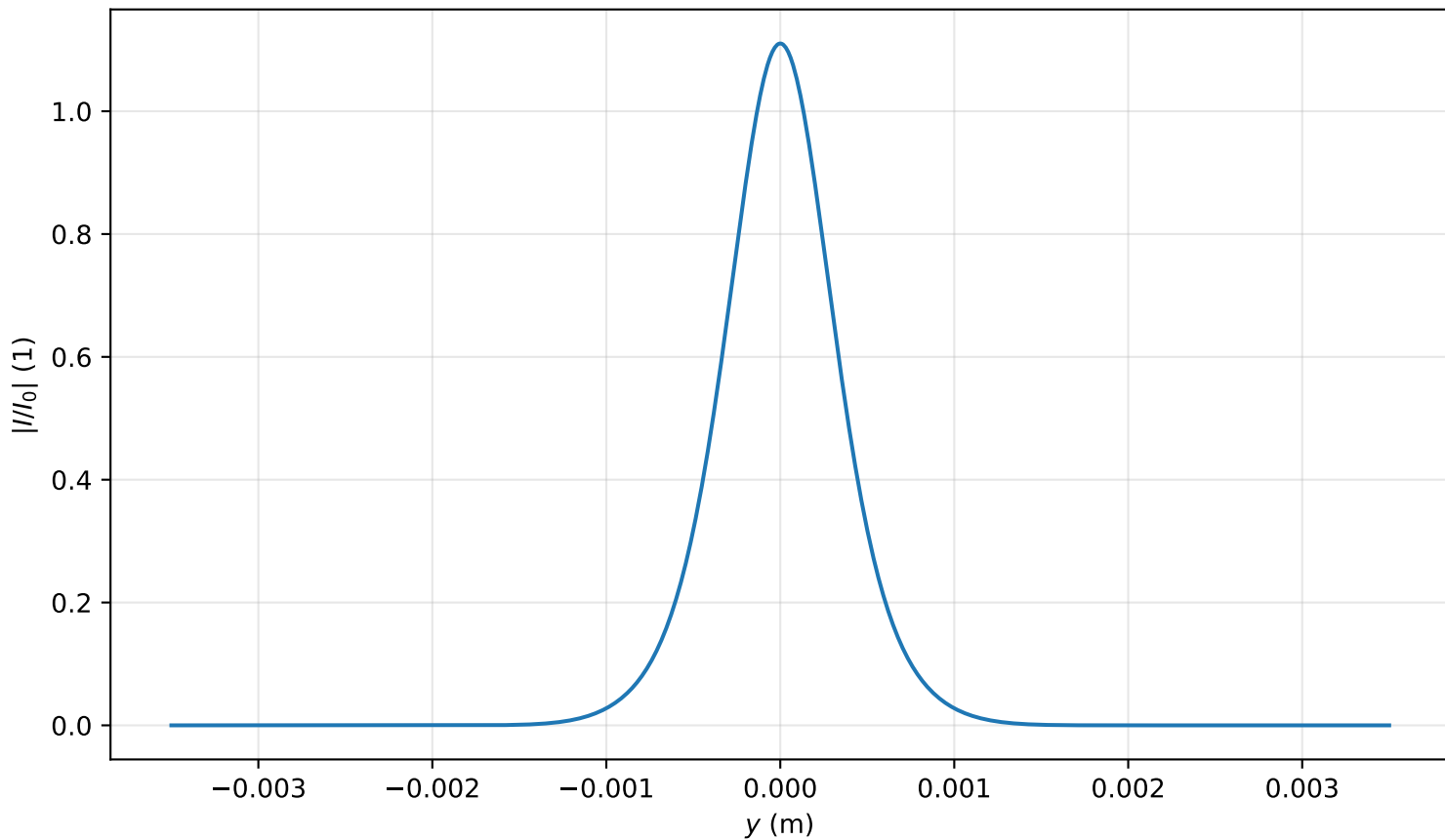
Intensity profile I(x=0, y, z=1.194)/I_0 , \text{Pin}=0.6P_{\text{cr}} , artificial time
